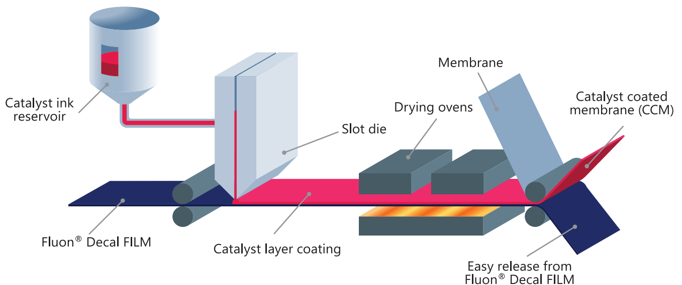
Schematic interpretation of the CCM production process
